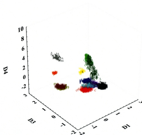
FIG. S2. A-C. Three-dimensional scatter plot of the multidimensional scaling performed with the complete data set of qualitative data. A. D1-D2-D3. B. D1-D2-D4. C. D1-D3-D4. Black (R), ROS populations of S. rosmarinifolia subsp. rosmarinifolia ; pale blue (B), S. rosmarinifolia subsp. arrabidensis ; violet (H), HET populations of S. rosmarinifolia subsp. rosmarinifolia ; red (C), S. canescens ; dark blue (S), S. semidentata subsp. semidentata ; yellow (M), S. semidentata subsp. melidensis ; orange (I), S. impressa ; grey (A), S. ageratifolia ; olive green (P), diploid cytotype of S. pectinata ; brown (T), tetraploid cytotype of S. pectinata ; pale green (O), S. oblongifolia ; dark green (L), hybrid complex between S. rosmarinifolia subsp. rosmarinifolia , S. oblongifolia and their putative hybrids.
