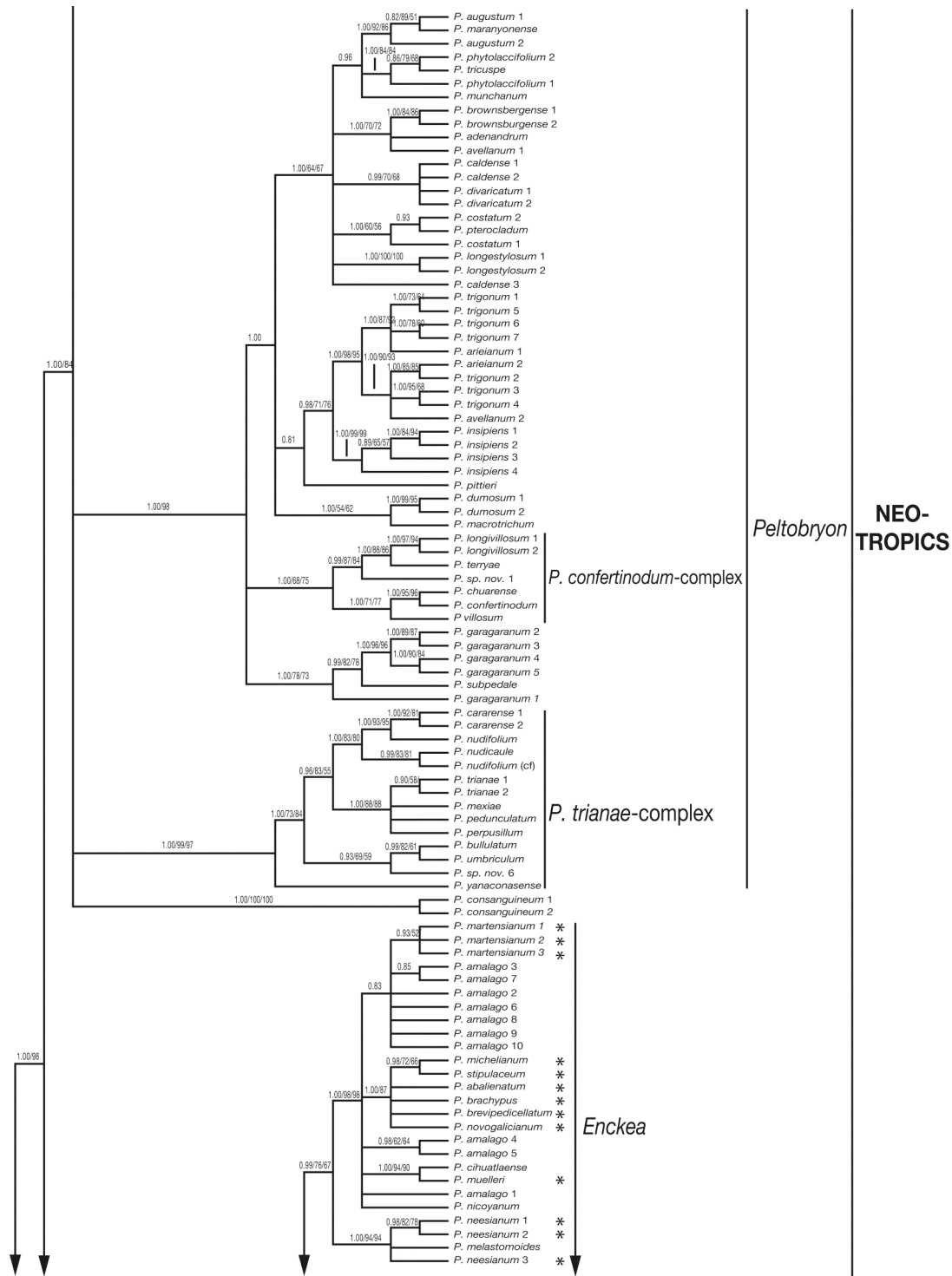
SUPPLEMENTAL FIG. 1D. Eighty percent majority rule consensus of the Bayesian analysis of the ITS sequences from Fig. 1. Numbers above branches indicate Bayesian posterior probabilities (B-PP), bootstrap values (>50% are shown) for maximum likelihood (BS-ML) and maximum parsimony (BS-MP) analyses (B-PP/BS-ML/BS-MP). African species are indicated with an arrow.
