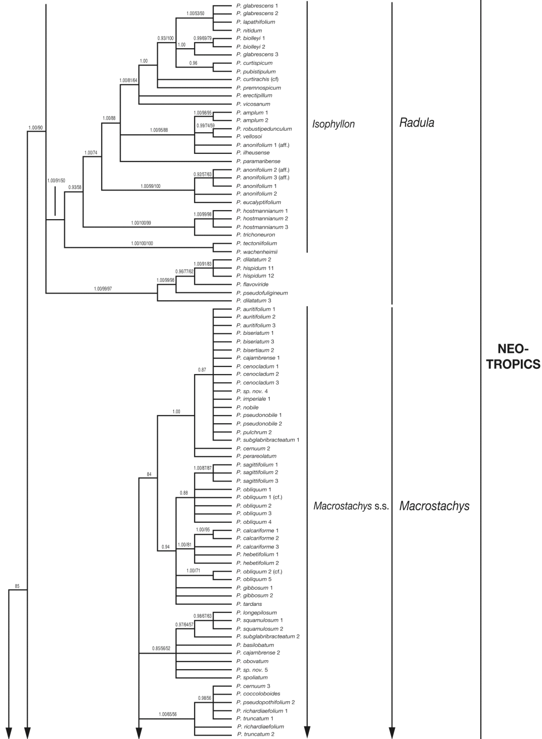
SUPPLEMENTAL FIG. 1B. Eighty percent majority rule consensus of the Bayesian analysis of the ITS sequences from Fig. 1. Numbers above branches indicate Bayesian posterior probabilities (B-PP), bootstrap values (>50% are shown) for maximum likelihood (BS-ML) and maximum parsimony (BS-MP) analyses (B-PP/BS-ML/BS-MP). African species are indicated with an arrow.
